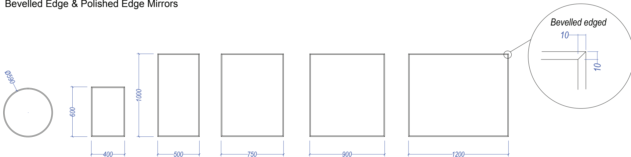
Bevelled edged mirrors with rear mounted brackets for fixing
