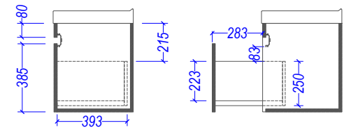
Suits "P" or "Bottle" Traps
