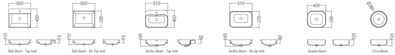
Sirocco bench tops to suit Slab & Serifos basins
